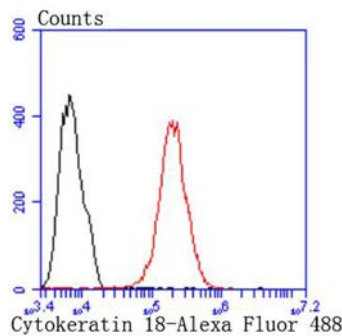
Fig. 3. Flow cytometric analysis of MCF-7 cells with Cytokeratin 18 antibody at 1/50 dilution (red) compared with an unlabelled control (cells without incubation with primary antibody; black). AlexaFluor 488-conjugated goat anti rabbit IgG was used as the secondary antibody.
